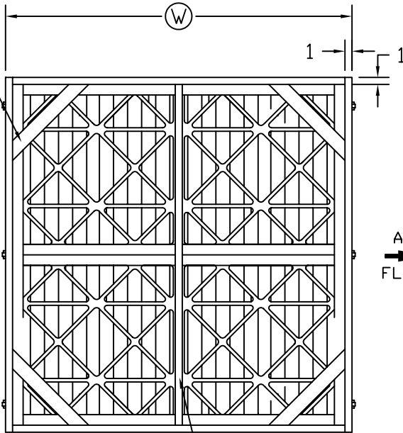
UPSTREAM SIDE
